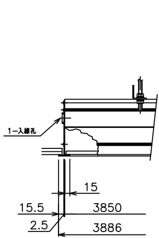
"a"部詳細
