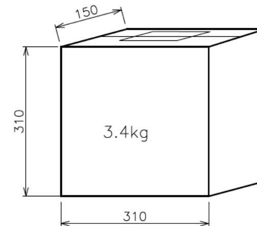
Packing size(1/8)
